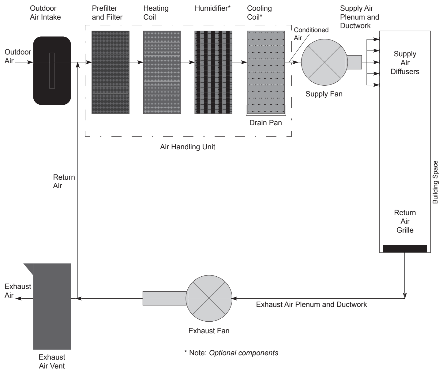
Figure A. General HVAC System Layout
