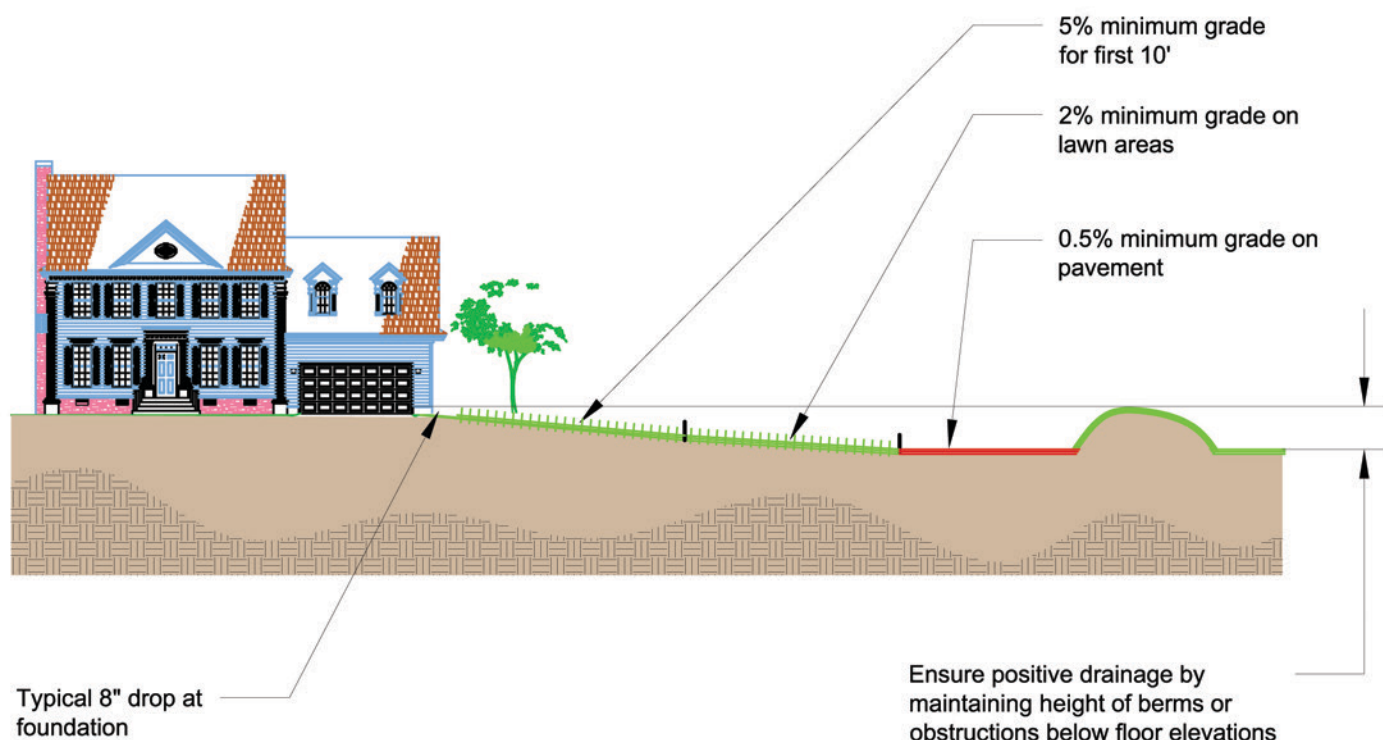
Figure 2-1 Positive Drainage Principles
